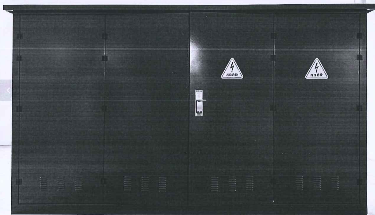
预装式金属封闭环网箱 (GHHW-JX-12)
