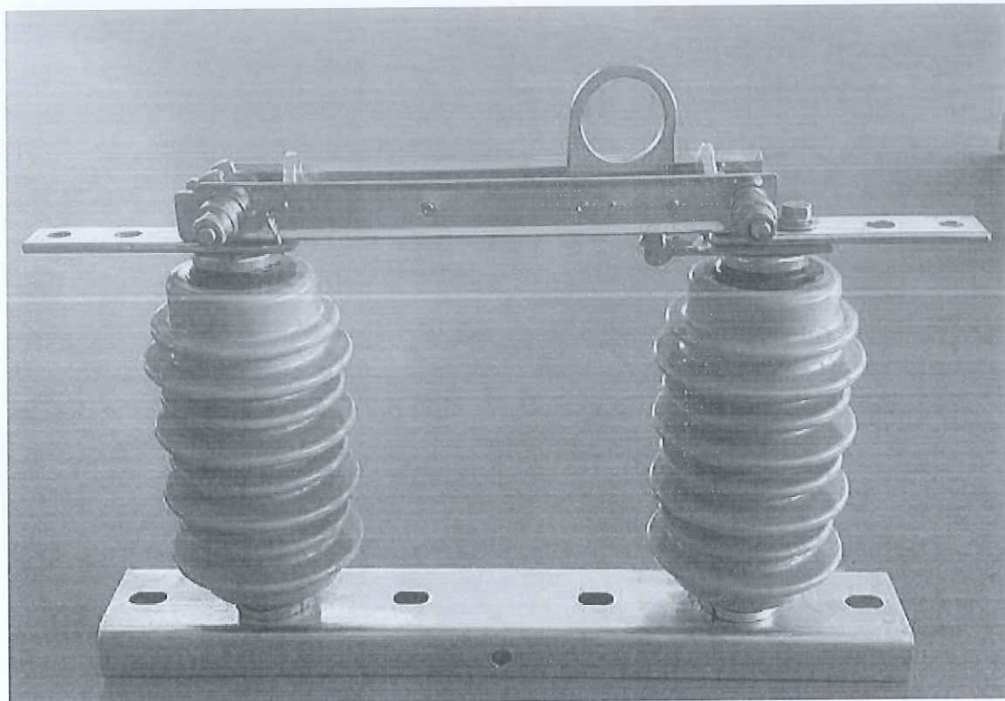
户外高压隔离开关 (GW9-12/630-20)
