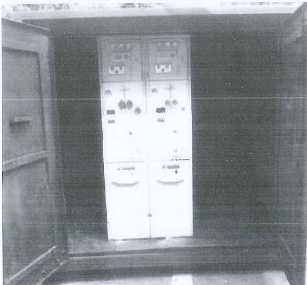
环网箱(箱式开闭所) (BSHWX-12 )
