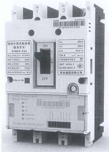
塑壳外壳式断路器(量测开关) (CAM5E-250LC)
