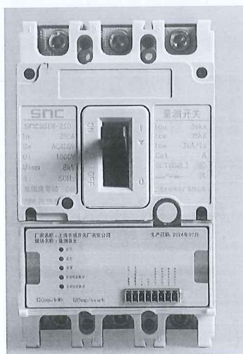
塑料外壳式断路器(量测开关) (SnCM8EW-250)
