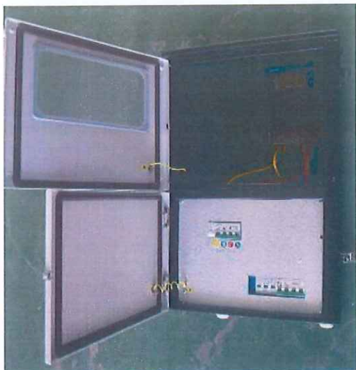
并网箱 (SHLX-BL30)
